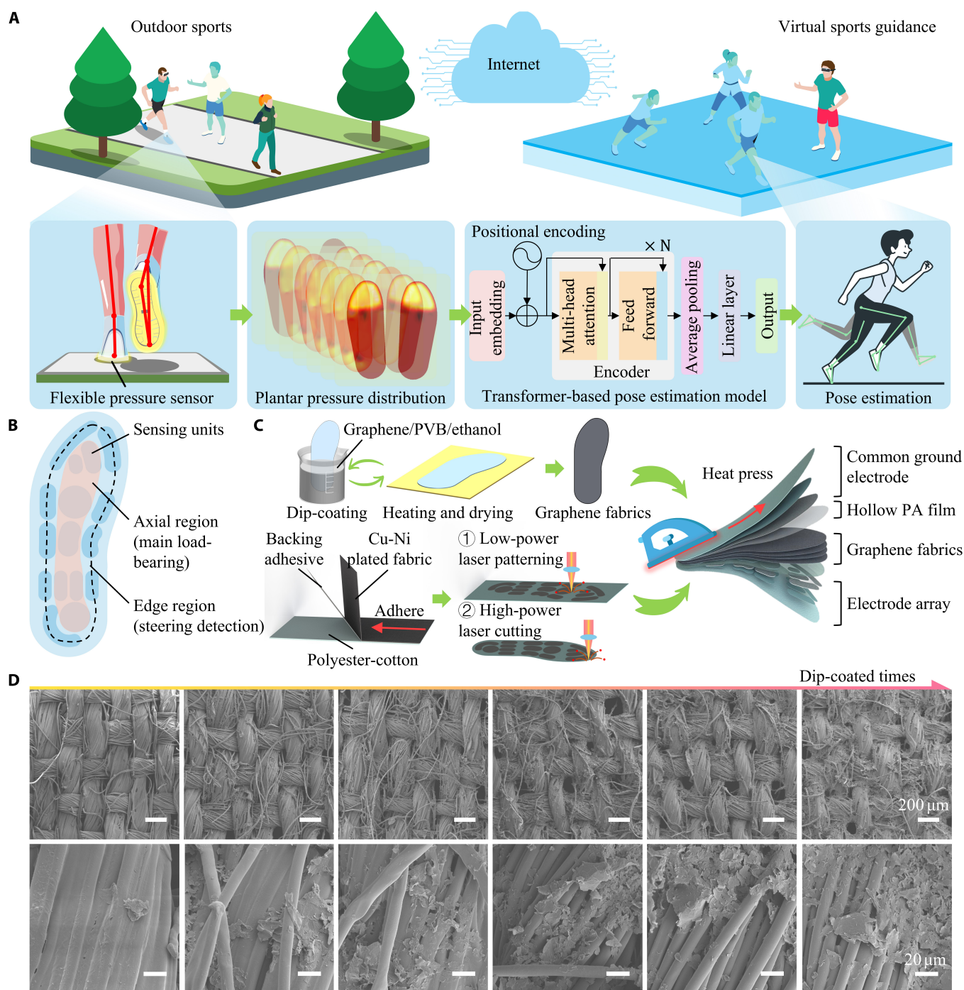
Fig. 1. Overview of lower limb motion capture system using fabric-based flexible pressure sensor array. (A) Workflow of the developed lower limb motion capture system. Plantar pressure signals are collected using 2 flexible pressure sensor array insoles. These signals are then processed by a transformer-based regression model to estimate the user's lower limb joint postures. The estimated postures are rendered within the next-generation Internet, enabling seamless and natural human-computer interaction. (B) Design of the flexible pressure sensor array. The insole-shaped flexible pressure sensor array, designed based on the plantar shape and pressure distribution principles, includes an axial region and an edge region. The axial region detects the primary weight-bearing areas during most postures, and the edge region detects the precise direction of force in most change-of-direction postures. (C) Fabrication process of the flexible pressure sensor array. The sensitive layer was formed by repeatedly dip coating the fabric with a conductive coating, and electrodes were patterned through laser selective cutting. The flexible pressure sensor arrays were fabricated via heat-pressing encapsulation. (D) Microstructural images of polyester cotton samples, ranging from untreated to those subjected to 5 dip-coating cycles.
