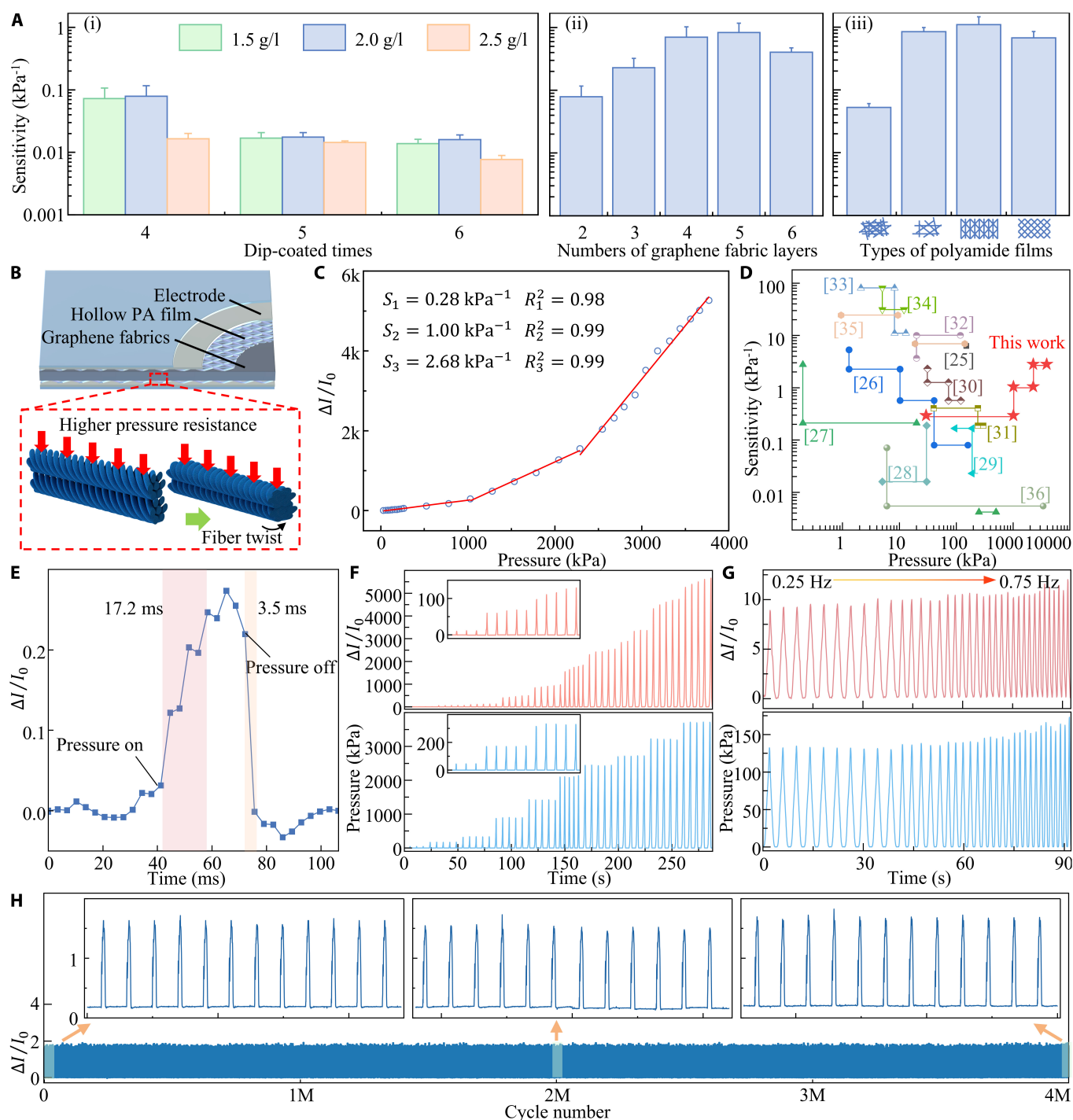
Fig. 2. Optimization of the piezoresistive performance of the sensing unit. (A) Influence of various preparation parameters on the performance of the flexible pressure sensing unit: (i) dip-coated times and concentrations; (ii) number of graphene fabric layers; (iii) types of PA films. (B) The designed sensing unit demonstrates an ultra-wide pressure range, attributed to the uniform PA film serving as a stable support and bonding structure, as well as the fiber twisting of polyester cotton fibers under stress. (C) Performance of the flexible pressure sensing unit using the optimal preparation parameters. (D) Comparison of the pressure range and sensitivity with previously reported fabric-based flexible pressure sensors. (E) Response and recovery times of the flexible sensing unit under rapid stimulation. (F) Sensing unit response under different pressure levels. (G) Sensing unit response to different pressure frequency. (H) Stability of the sensing unit over 4 million loading/unloading cycles.
