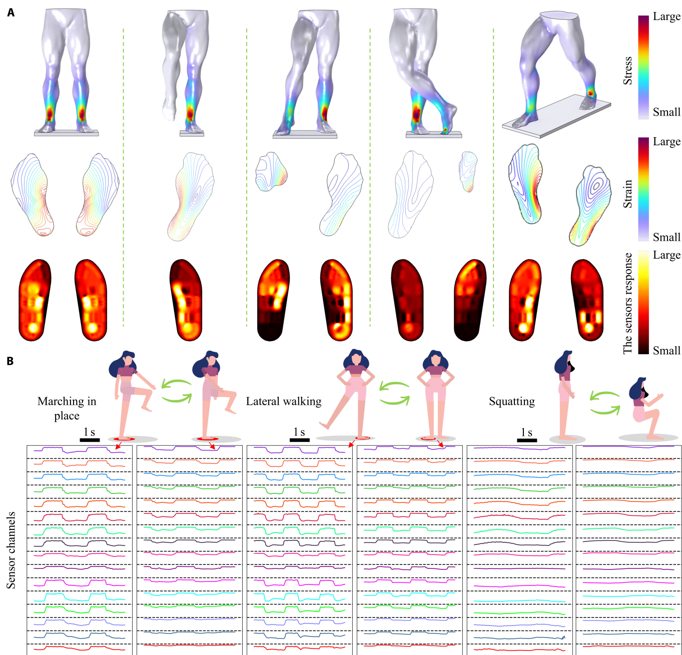
Fig. 3. Testing of the flexible pressure sensor array insole. (A) Simulated plantar pressure distributions and sensor array test results under various lower-body postures. (B) Response curves of the flexible pressure sensor array insole during marching in place, lateral walking, and squatting.
